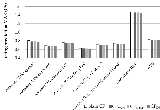
Figure 9. Rating prediction MAE for the datasets summarized in Table 4, when the CS user similarity metric is used.
